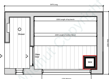
01 Vesi - With Porch and Shower - GA Plan (With 9 KW Sauna Heater)
